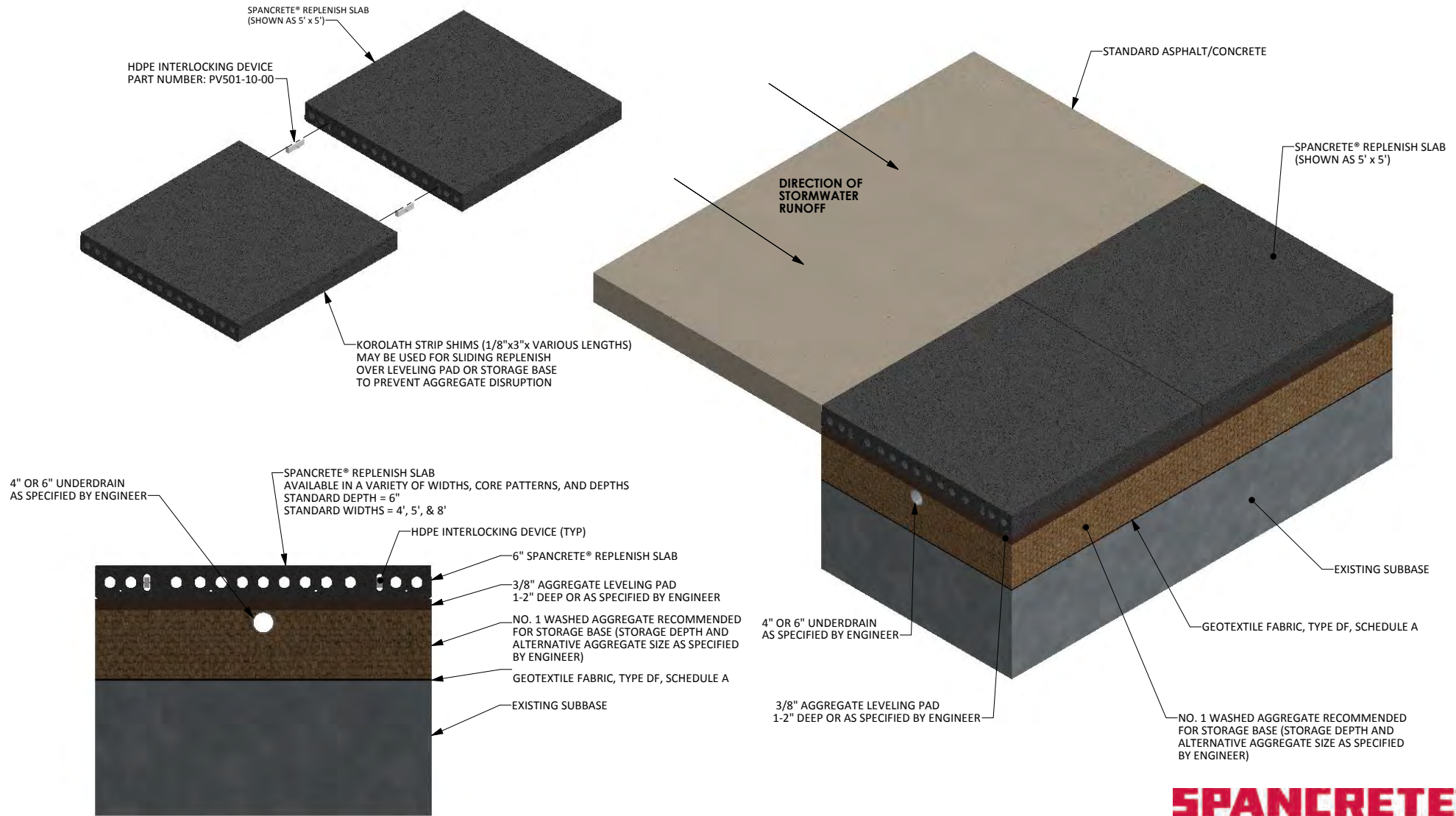
CROSS SECTION WITH STANDARD CORE PATTERN FOR 5' WIDE SPANCRETE® REPLENISH SLAB
