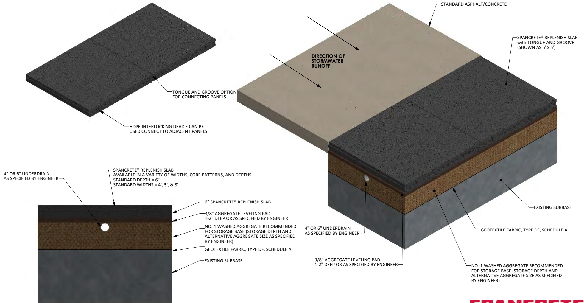
CROSS SECTION WITH STANDARD CORE PATTERN AND TONGUE AND GROOVE FOR 5' WIDE SPANCRETE® REPLENISH SLAB
